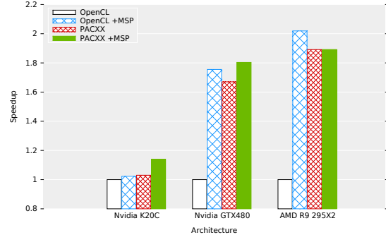
Figure 2: Speedup of PACXX over OpenCL with and without multi-staging for parallel reduction, input off 2^{27} integers.
