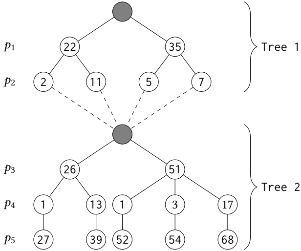
Fig. 1. The example chain-of-trees represents the search space of parameters p_1, \dots, p_5 .
