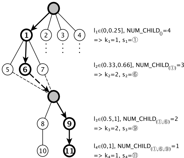
Fig. 2. Example of exploring our chain-of-trees structure in multiple dimensions, based on an L -dimensional coordinate space (in this example: L = 4 ). Subtrees in level 1 – for nodes 2, 3, 4 – are omitted for brevity.
